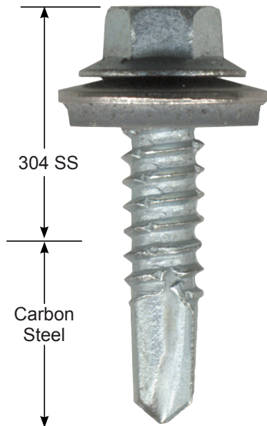
Bi-Metal Screws
